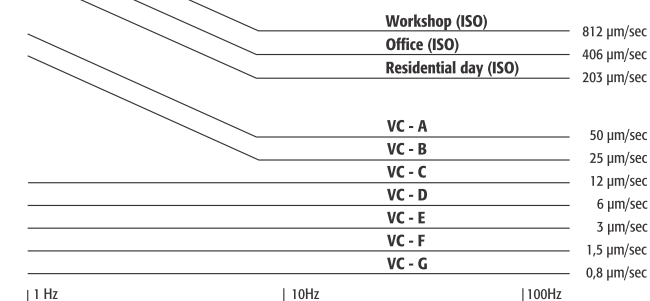
Chart 2: Vibration Criteria VC
