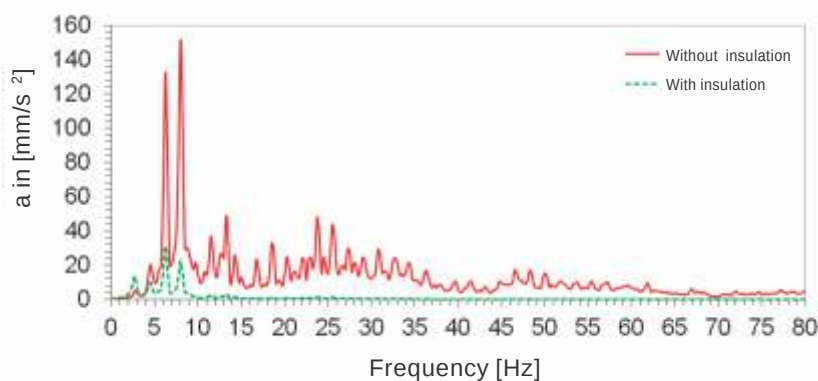
With/without insulation
